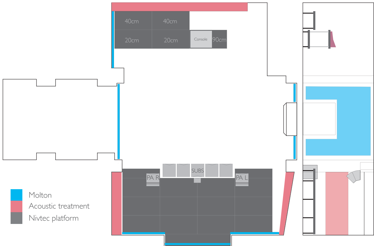
Picture. 1a. Ground plan | CONCERT MODE.
