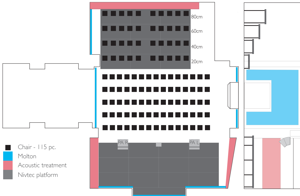
Picture. 1b. Ground plan | FILM / THEATRE MODE.
